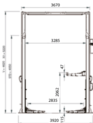
PDCH45C Symmetric Installation
