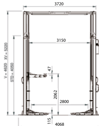
PDCH55C Asymmetric Installation
